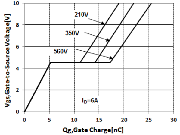
Fig 10 Gate-Charge Characteristics
