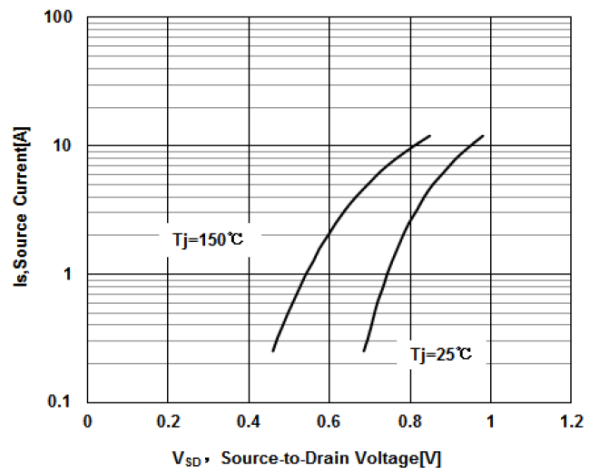
Fig 6 Body-Diode Characteristics
