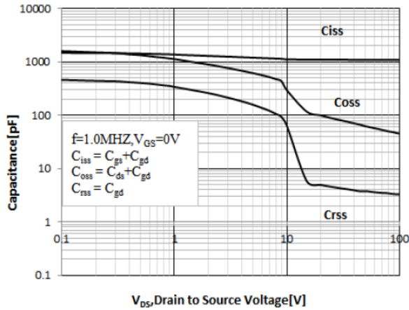
Fig 9 Capacitance Characteristics
